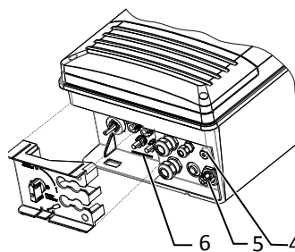
Fig. 10: Surveying the connection area
