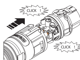
Fig. 16: Press contact carrier into the housing
