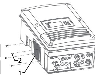
Afb. 27: Ventilator demonteren
