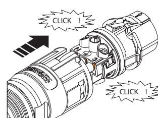
Afb. 16: Contactdrager in behuizing duwen
