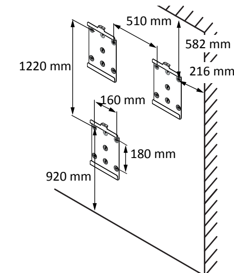
III. 8: Montage mural
