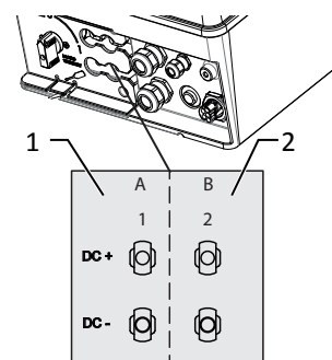
Fig. 24: Connection for DC positive and DC negative
