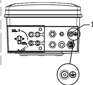
Afb. 25: Extra aardingspunt
