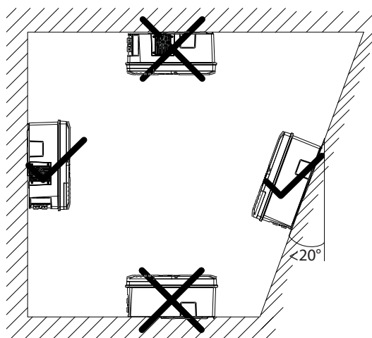
Fig. 4: Permissible installation location
