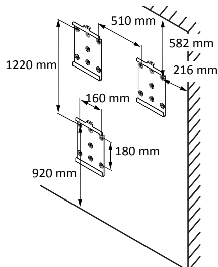
Afb. 8: Wandmontage
