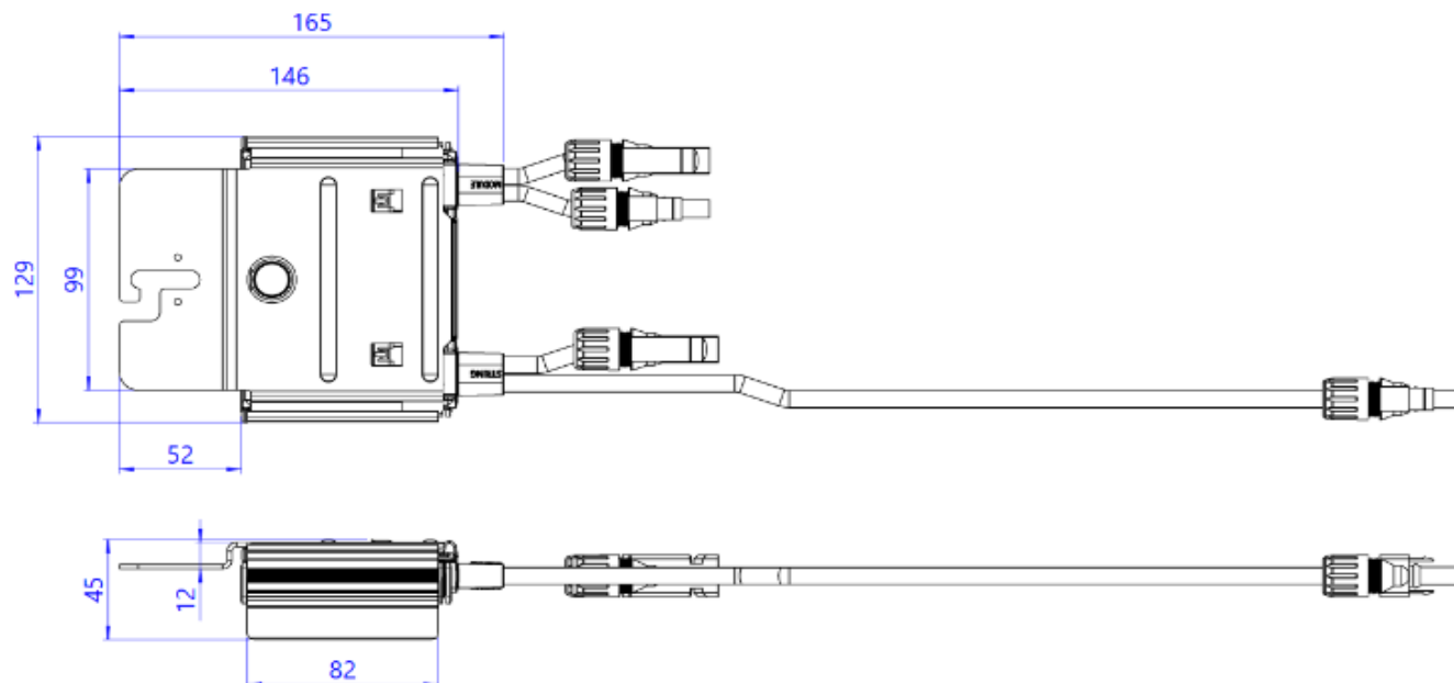
S650A (Bent Bracket)
